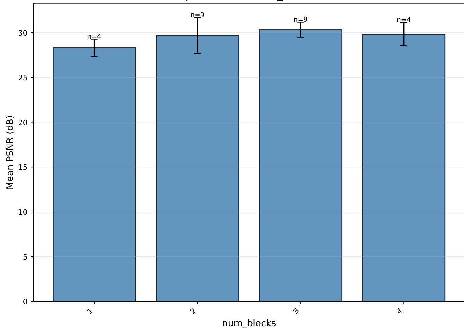
Mean PSNR per value of num_blocks — OmniSR
